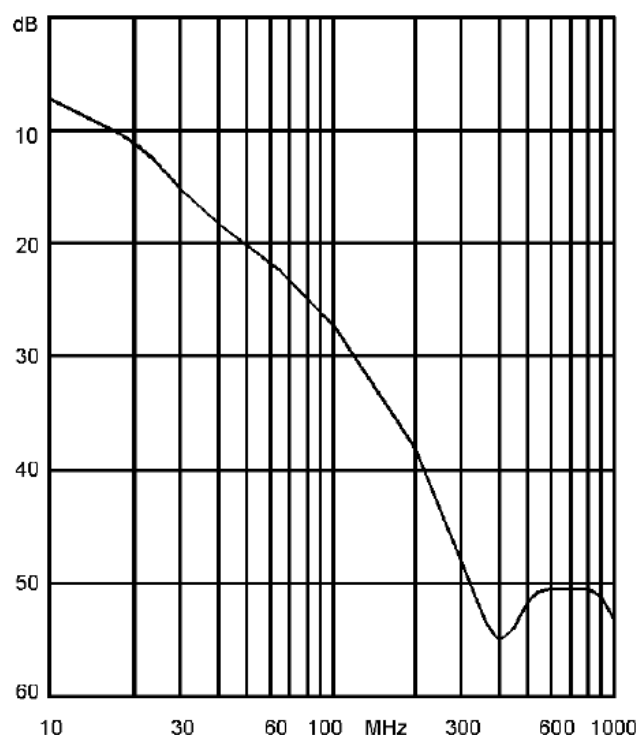
Typical Loss vs. Frequency (50 ohm line)
