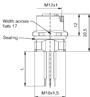
Female connector, M16x1.5 thread, front panel mounting, wire termination
