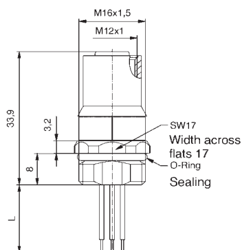
Female connector with LED, M16x1.5 thread, front panel mounting, wire termination
