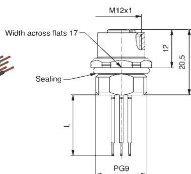
Female connector, PG9 thread, front panel mounting, wire termination
